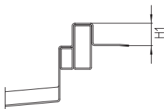
AF Attachment flange 1)
