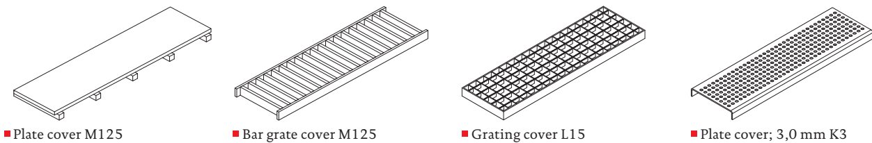
■ Plate cover M125 ■ Bar grate cover M125 ■ Grating cover L15 ■ Plate cover; 3,0 mm K3
