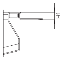
HF Bonding flange 1)
