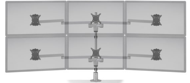
STAXX THREE OVER THREE WIDE Screen Size: 24" - 30" Weight Capacity: Up to 10 lbs. per monitor Part Number: STX-33W-___
