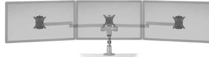
STAXX TRIPLE WIDE Screen Size: 24" - 30" Weight Capacity: Up to 15 lbs. per monitor Part Number: STX-03W-___
