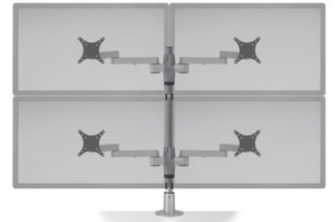
STAXX TWO OVER TWO WIDE Screen Size: 24" - 30" Weight Capacity: Up to 15 lbs. per monitor Part Number: STX-22W-___
