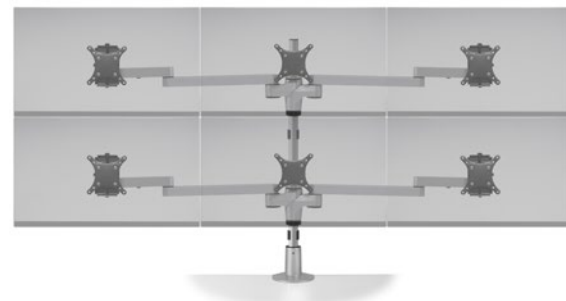
STAXX THREE OVER THREE Screen Size: Up to 24" Weight Capacity: Up to 10 lbs. per monitor Part Number: STX-33S-___
