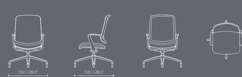
Upholstered - Four Star Base Gliders
