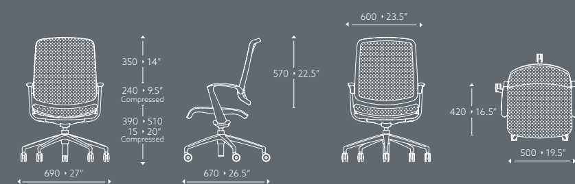
Mesh - Five Star Base Castors
