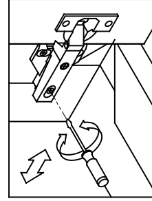
FIG D DEPTH ADJUSTMENT
