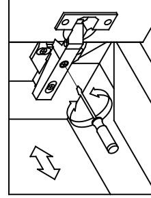
FIG C SIDE ADJUSTMENT
