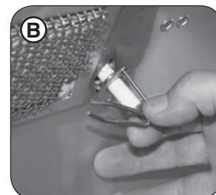
Fig. 31-2 Remove electrode
