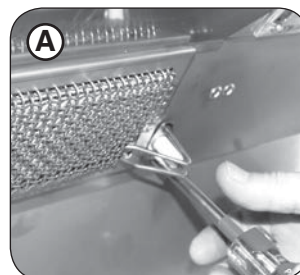
Fig. 31-2 Remove electrode
