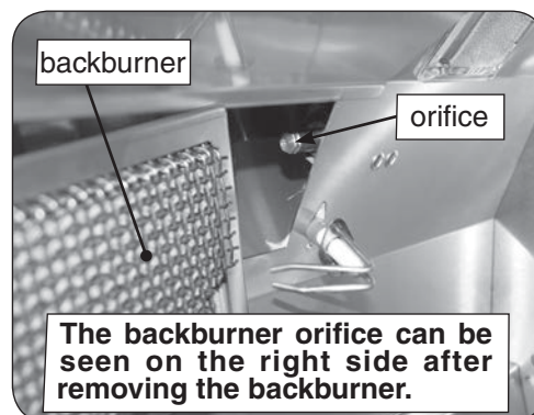
Fig. 31-4 Remove backburner
