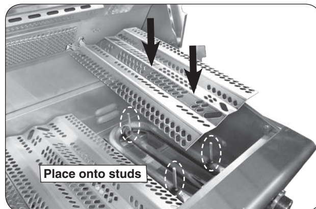
Fig. 22-1 Install vaporizer panels
