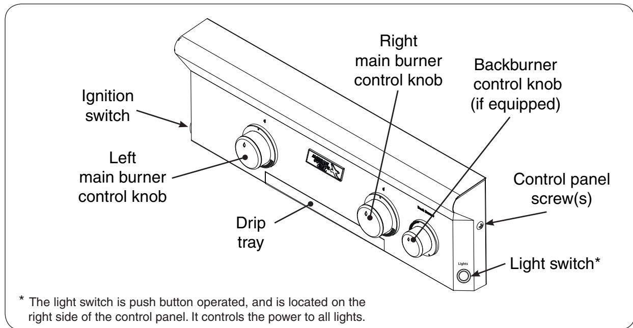
Fig. 24-1 Grill controls
