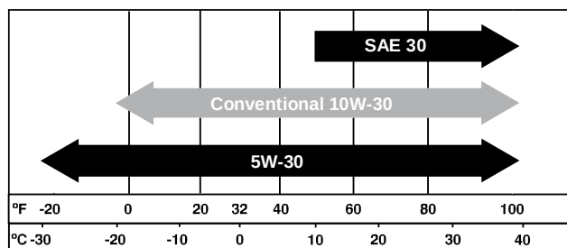
Figure 25 – Recommended Oil
