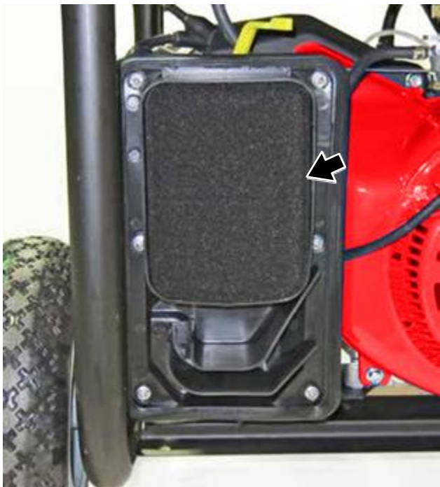
Figure 31 – Removing Coarse Outside Air Filter
