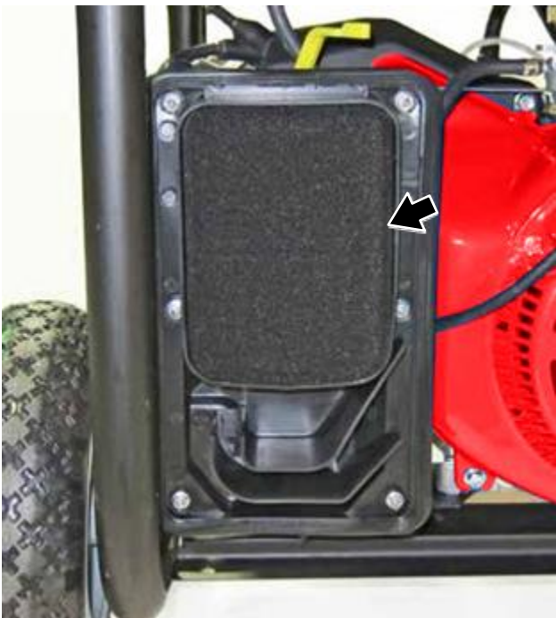
Figure 31 – Removing Coarse Outside Air Filter
