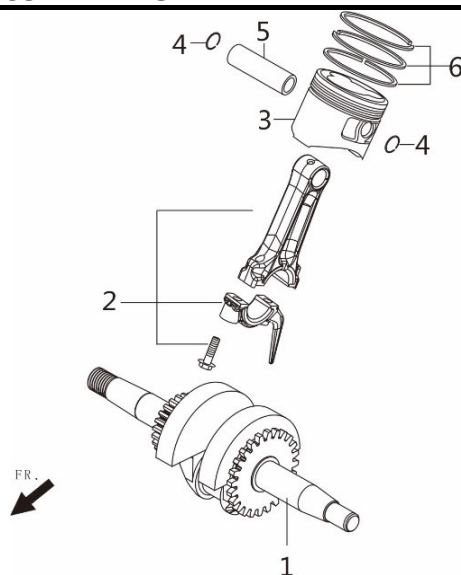
FIG.3 RING SET,OIL / ROD,CRANKSHAFT CONNETING
