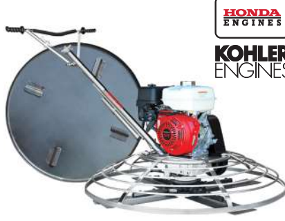
36" & 46" Concrete Power Trowel Part#: TPT36H/K & TPT46H/K
