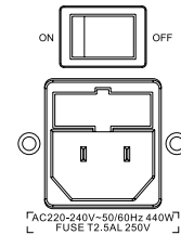
AC230-240V-50/60Hz 440W FUSE T2.5AL 200V
