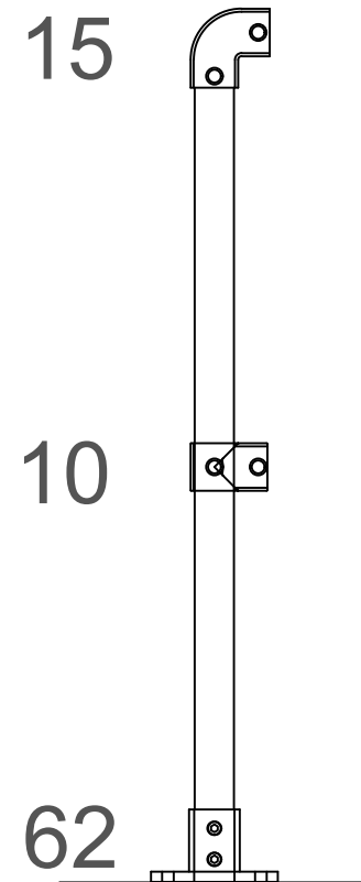
END POST
