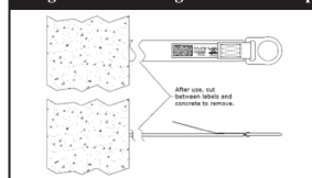
Figure 7 - Removing the Anchor Strap
