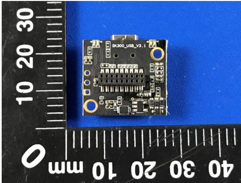
Photo 9 PCB view
