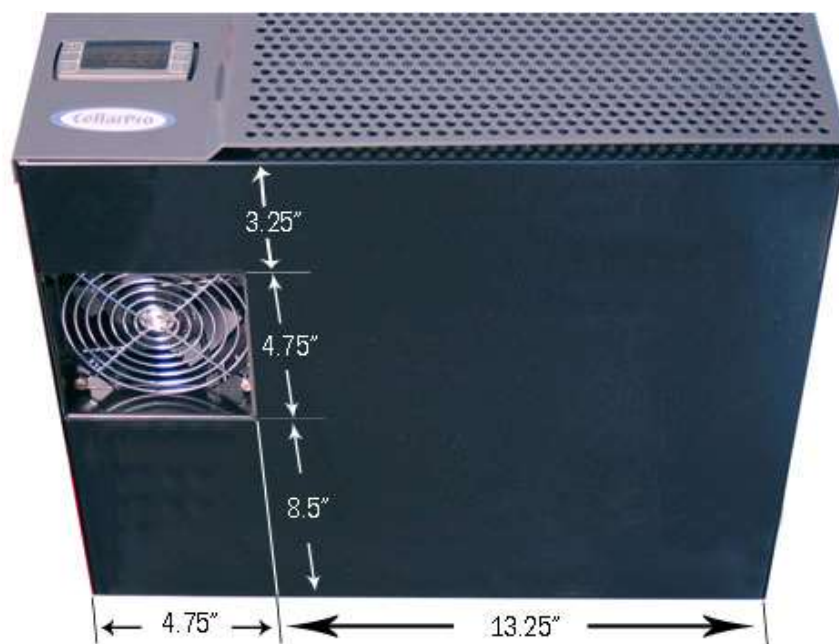
BOTTOM VIEW
