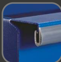
5 Double Hemmed Edges Drawer edges are hemmed to double thickness for extra stiffness.
