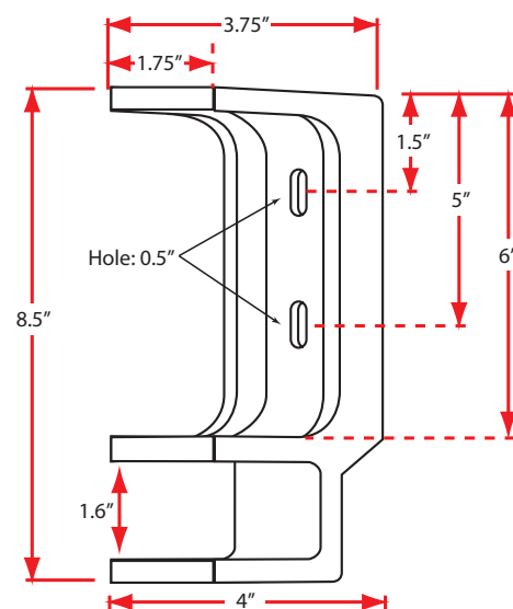
L series Dual-use Bracket
