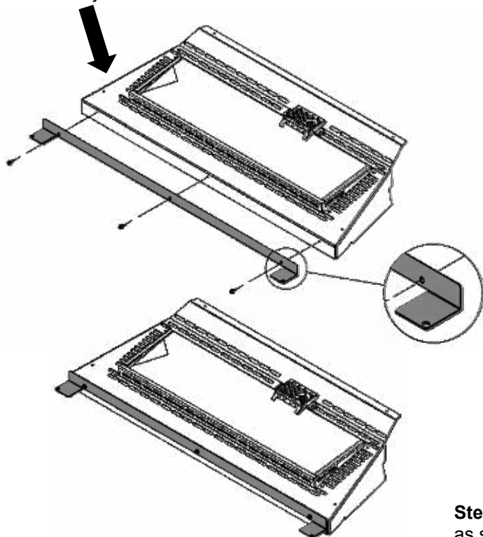
Step Two: Attach Front Fence to GT Glass Tray as shown.
