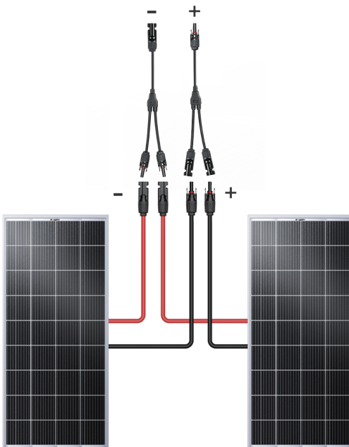
Parallel Connection
