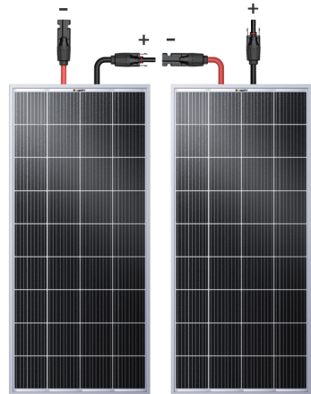
Electrical Connection
