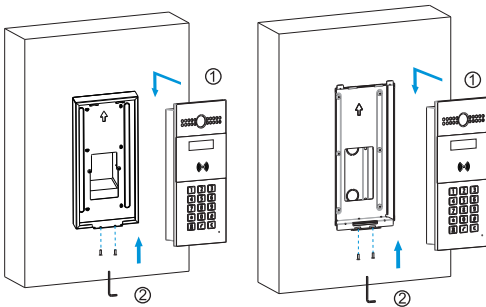
Wall Mounting
