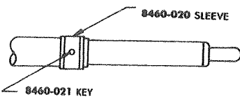
LOCK ADJUSTING PKG. 8460-0201. (Canvas Support Ass'y)
