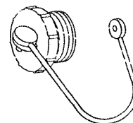
CITY FILL CAP & STRAP 4714-0481 for 4732B1521 and 4732C1521 City Fills
