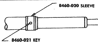
LOCK ADJUSTING PKG. 4714-5491 (Canvas Support Ass'ys.)
