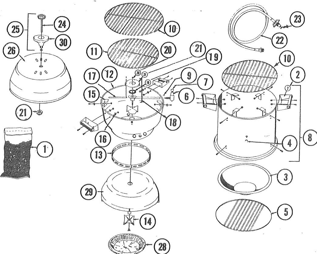
Gas Smoker Grill model 5475-701
