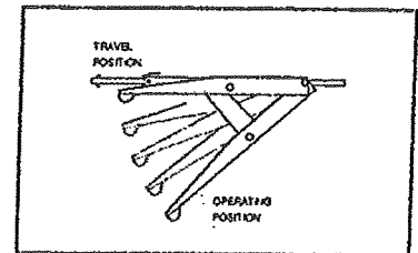
Crank-Down Stabilizer
