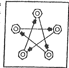
Torque Chart
