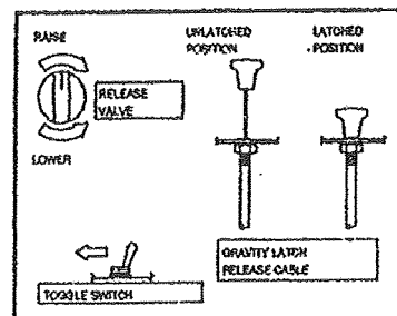
Power Lift Controls
