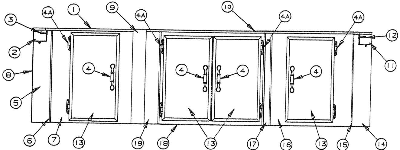
LOWER GALLEY ASSEMBLY (SHORT) - AMERICANA SERIES
