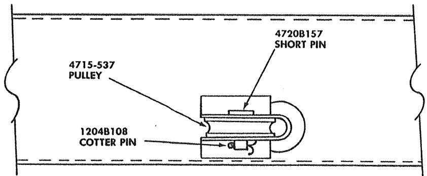
DETAIL B
