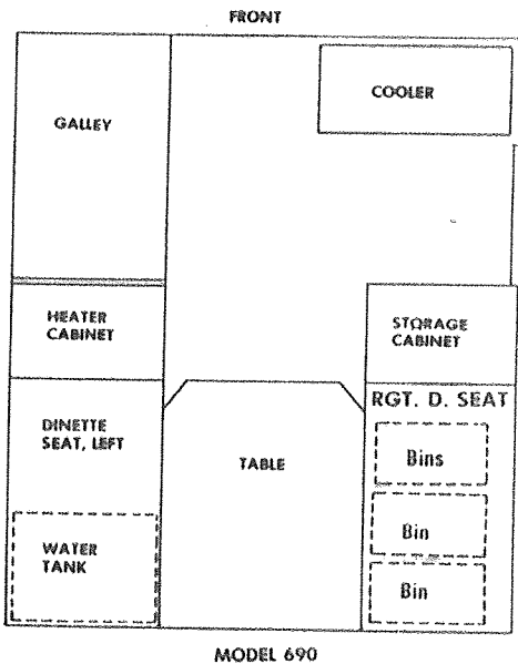
Figure 7 Floor Plan
