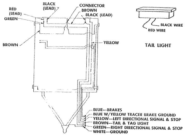
Figure 8 Wiring Diagram
