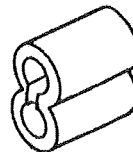
4720C169 CABLE CLIP USED ON LIFT AND WHIFFLE TREE CABLES USED ON 1/8" DIA. CABLE
