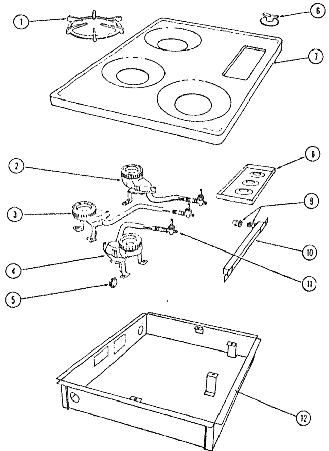
MODEL NO. 4710B0311 PAPRIKA RED STOVE
