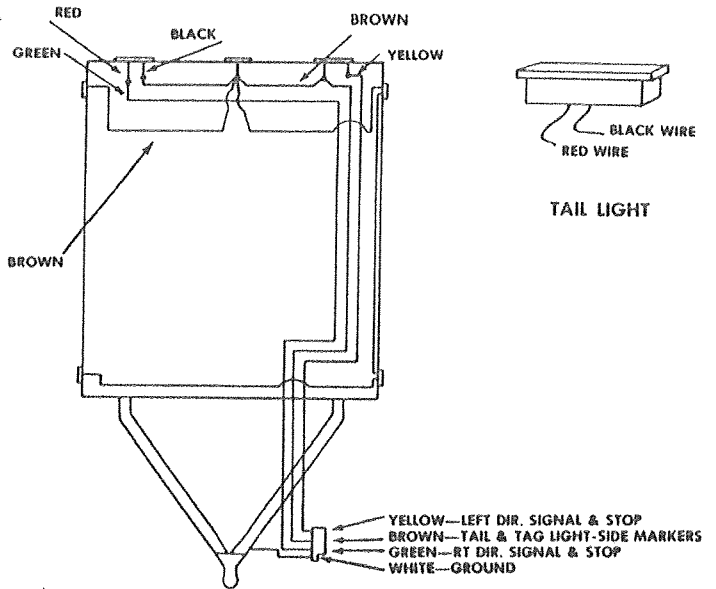
Figure 8 Wiring Diagram
