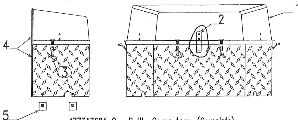
4773A7691 Gas Bottle Cover Assy. (Complete)
