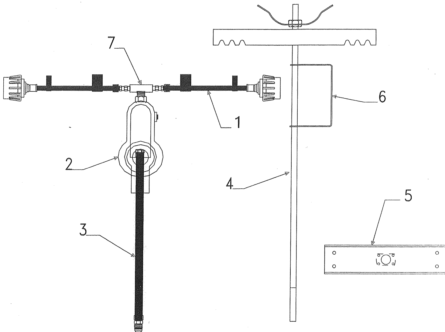
Dual Propane Tank Kit (4755B7801)
