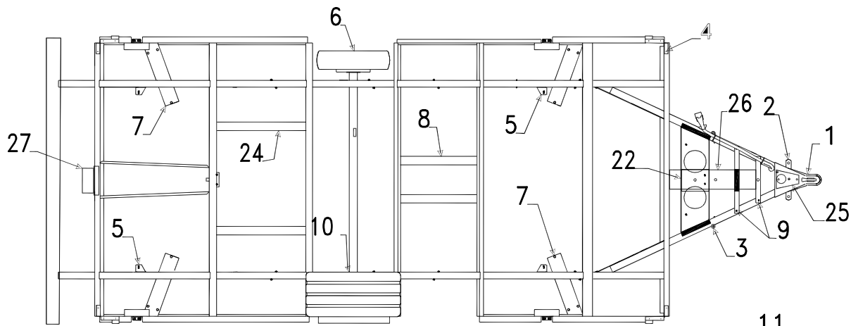
Frame Assembly Component Parts
