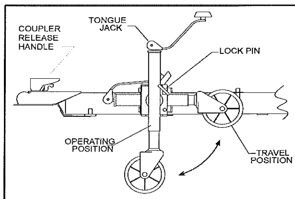
Tongue Jack
