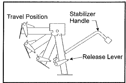
Swing-Down Stabilizer
