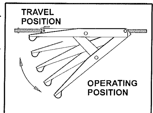
Crank-Down Stabilizer
