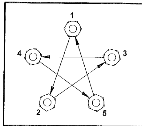
Torque Chart
