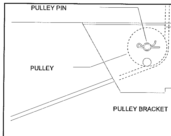
Adjustable Pulley
