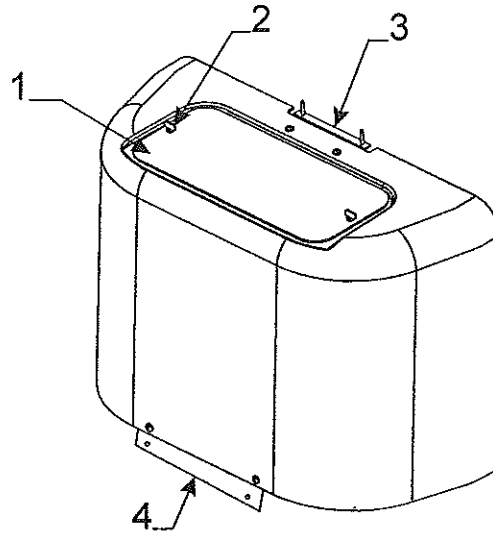
Molded Gas Bottle Cover Assembly (4749L1341)
