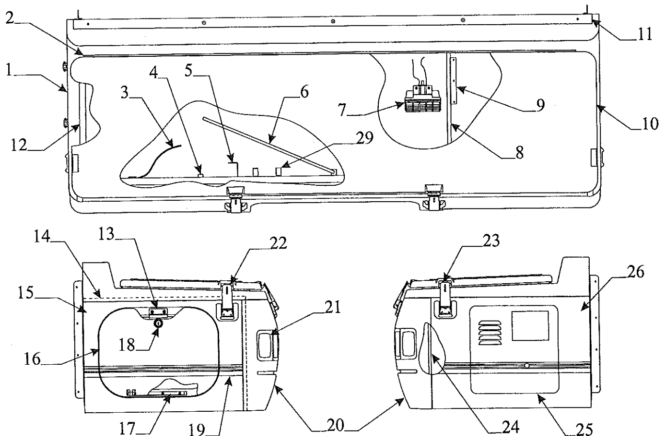
Storage box components - 3551,78,81,94,95,96
