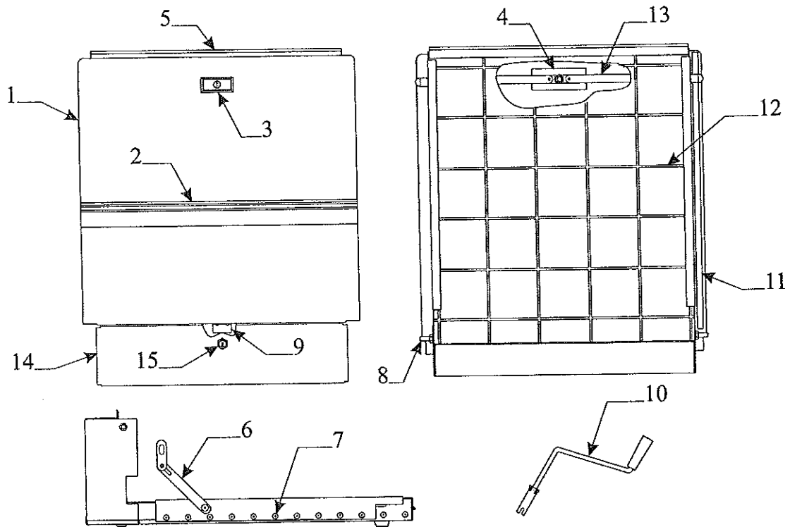
4754B6931 Access Door Assembly "complete" less trim tape FLAT RATE 1.25 complete door assembly
