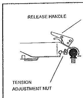
Coupler
