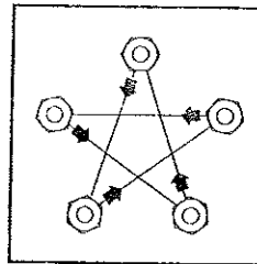
Torque Chart
