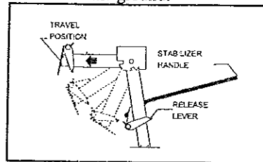
Swing-Down Stabilizer
