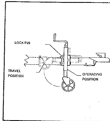
Tongue Jack
