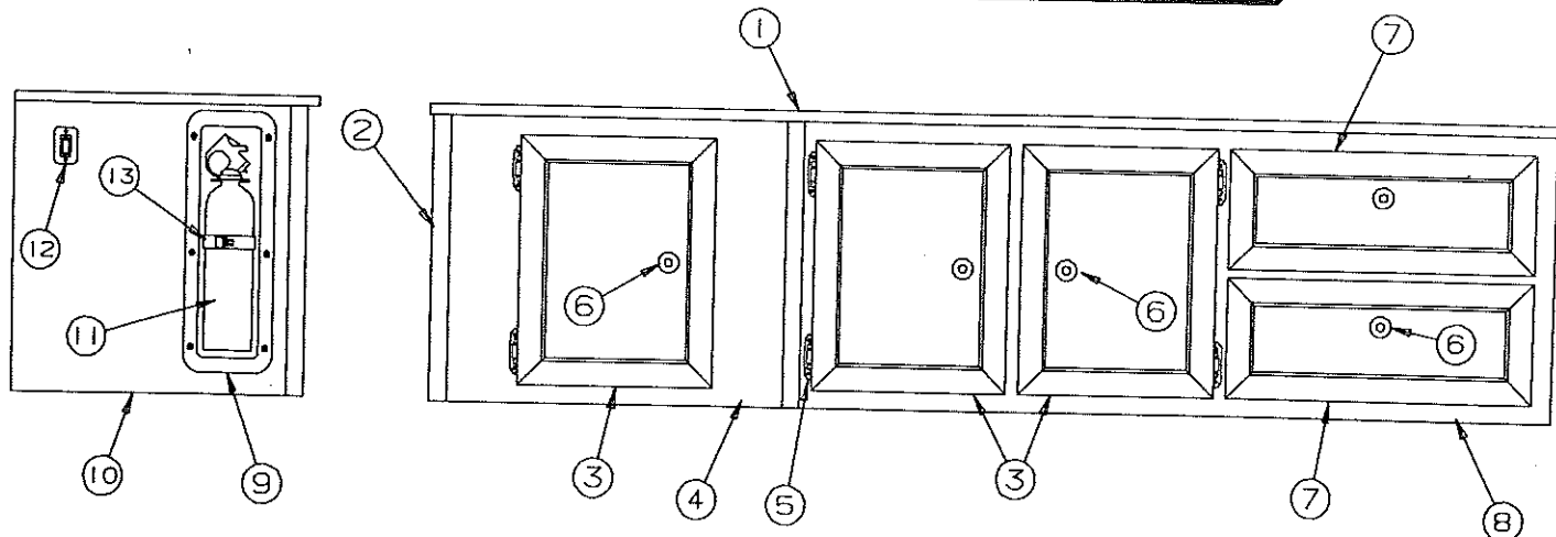
2993, 2998 HUTCH ASSEMBLY (4744H580)
