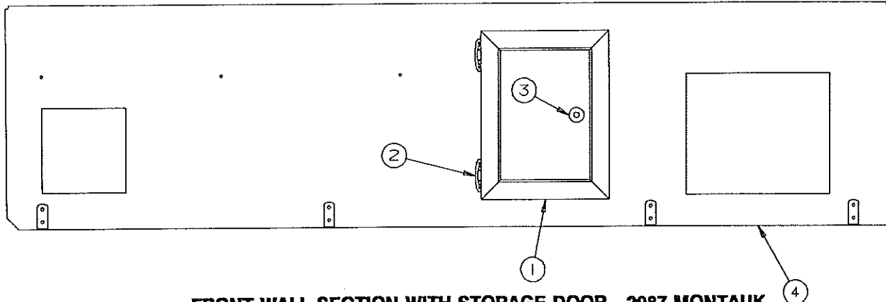
FRONT WALL SECTION WITH STORAGE DOOR - 2987 MONTAUK
