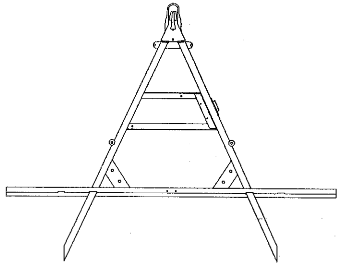
4716-1501 "A" Frame Assembly 2689 Royale
