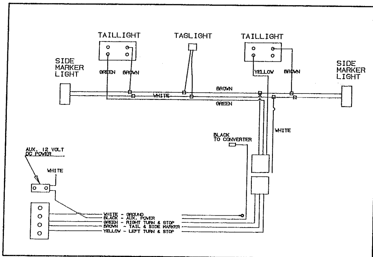
WIRING DIAGRAM - ROANOKE
