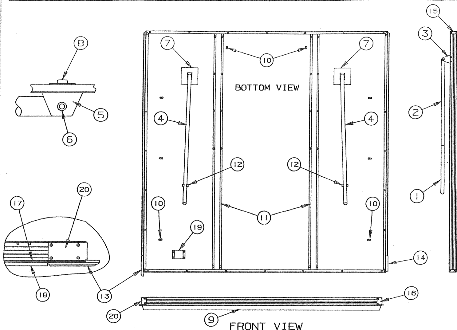
QUEEN BED ASSEMBLY 2489
