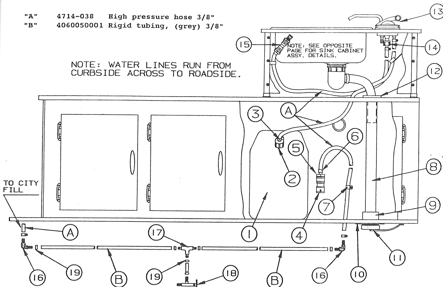
2470, 2489 DESTINY SERIES WATER SYSTEM
