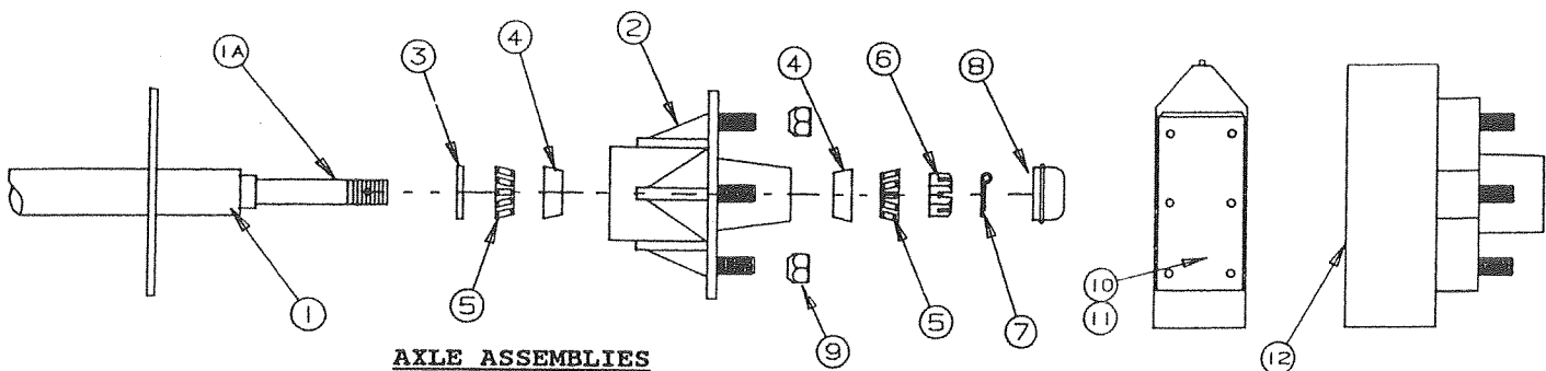
AXLE ASSEMBLIES
