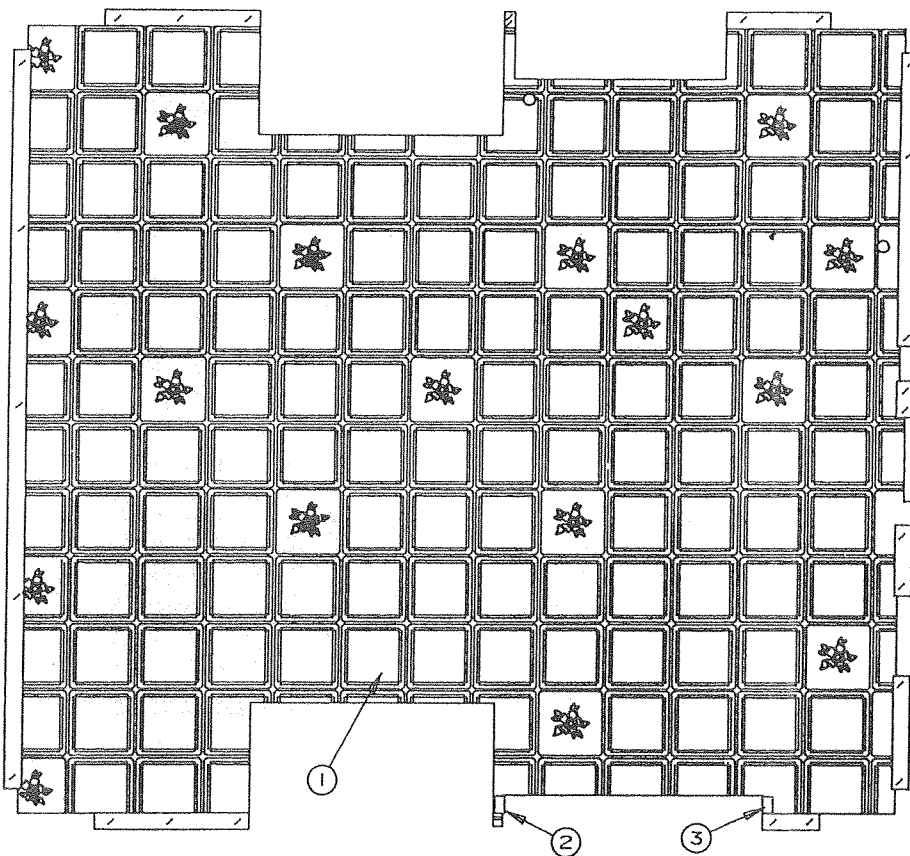
FLOOR ASSEMBLY, 2400 PIONEER
