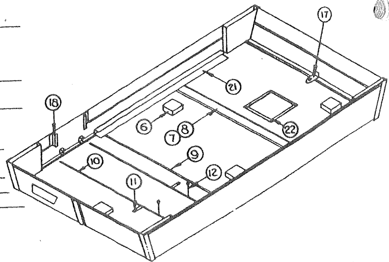
4745-3511 Lift cover (RSF/CSR) 4745-3501 Lift cover (RSR/CSF)
