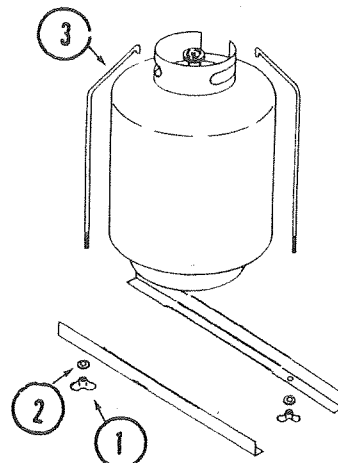
GAS BOTTLE BRACKET ASS'Y 4733F6281 (without block) 1 1201-625 Wing Nut 2 1202B043 Washer 3 4733A056 Mounting Brkt. Gas Bottle & Bottle Angles not in Pkg.
