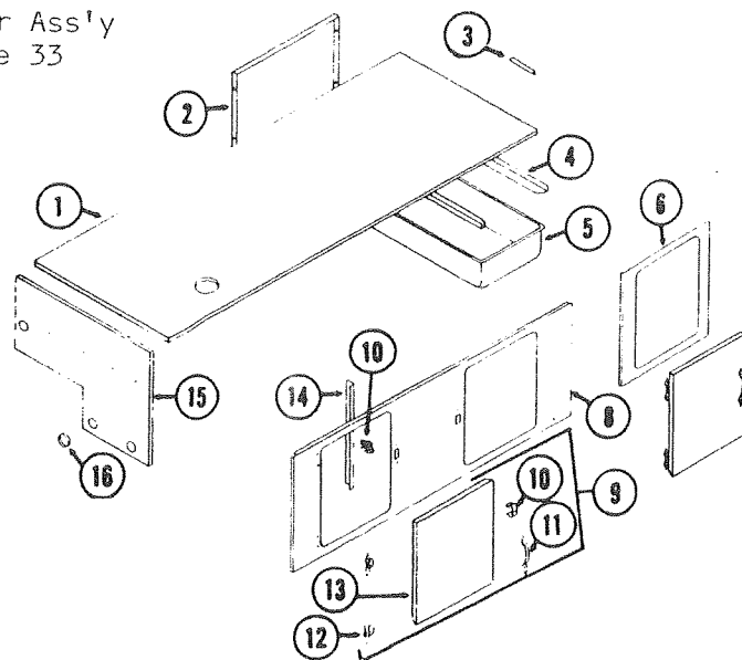
LOWER GALLEY ASSEMBLY, 4741-516, 1580, 1485
