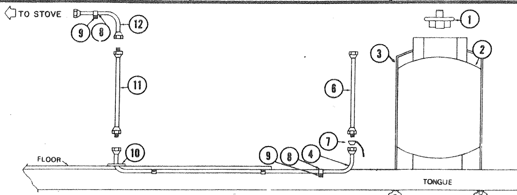
GAS SYSTEM, EXCEPT 1565, 1595
