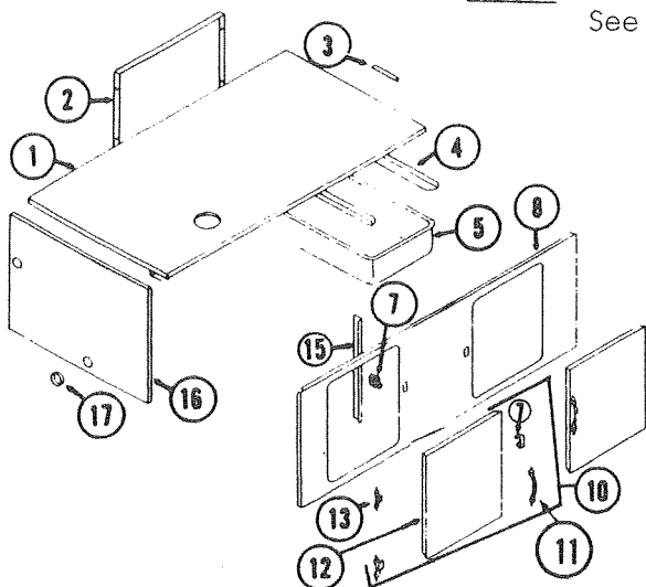
LOWER GALLEY ASSEMBLY, 4737D588, 1560 LOWER GALLEY ASSEMBLY, 4741-608, 1566
