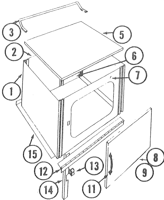
WORK CABINET ASS'Y, 4733G693, 1480, 1494, 1414 WORK CABINET ASS'Y, 4733F688, 1490, 1410
