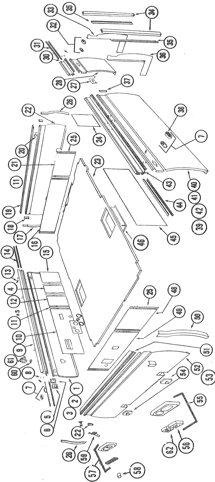
PANEL PARTS LIST--LIGONIER, 1460; AND REBEL 1465.
