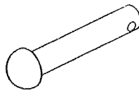
COUPLER HITCH PIN 4739-139 Ideal 1/4" Dia. 2 5/8" Lg., 3/8" Dia. Hd.
