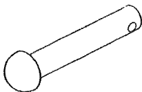
COUPLER HITCH PIN 4771-263 Fulton 5/16" Dia. 1 3/4" Lg., 1/2" Dia. Hd.
