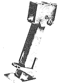
STABILIZER--ATWOOD 4714-4001 Stabilizer 4733-5951 Handle
