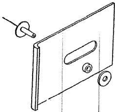
SCREEN DOOR SLIDE ASS'Y 4737-1921 1203-897 Rivet 1202B269 Washer 322-330 Aux. Valve Disc Washer 4737-192 Slide
