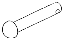
COUPLER HITCH PIN 4771-263 Ful-ton 5/16" Dia. 1 3/4" Lg., 1/2" Dia. Hd.
