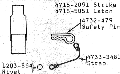
LATCH ASS'Y FOR PANELS This latch used on 800 Series.
