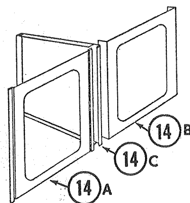
LATE MODEL 1060 WITH TWO-PART FRONT
