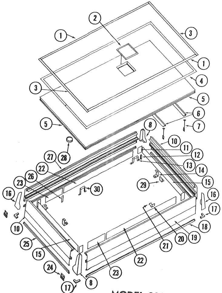
MODEL 890 SHOWN
