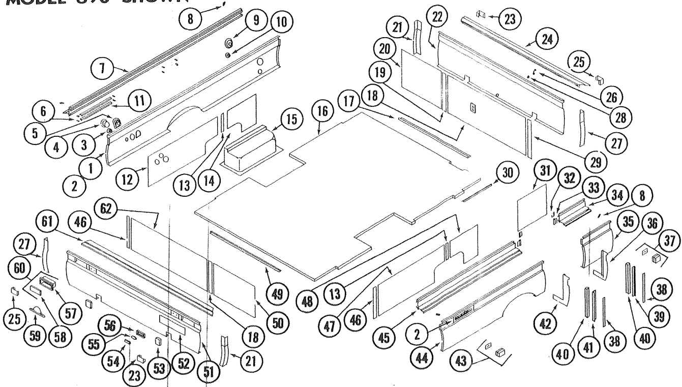
PANELS -- SOMERSET, MODEL 870
