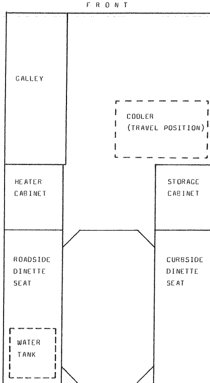
FLOOR PLAN
