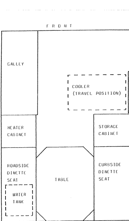
FLOOR PLAN
