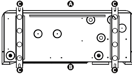
View of the appliance base from below for installing the anti-vibration pads
