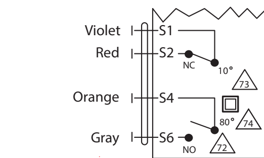
Auxiliary Switch
