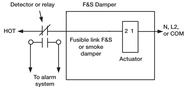
Typical smoke or fusible link damper wiring
