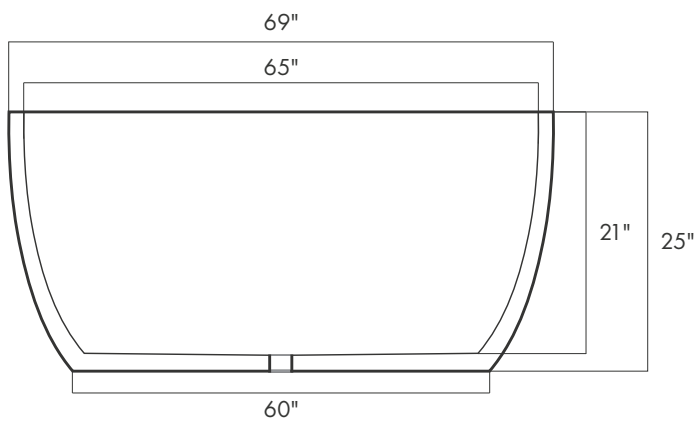
SECTION VIEW
