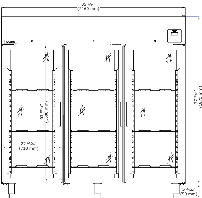
Front (Closed - Glass Door)
