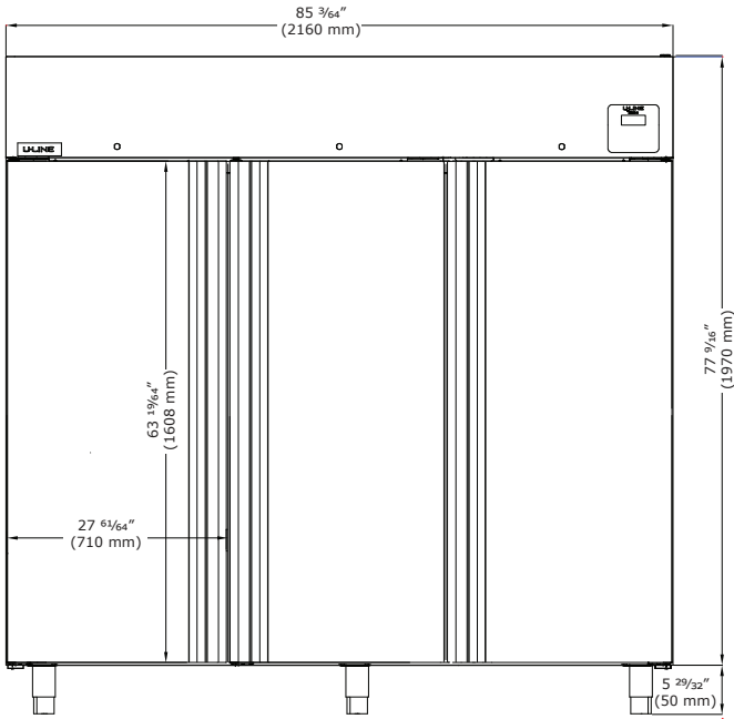
Front (Closed - Glass Door)
